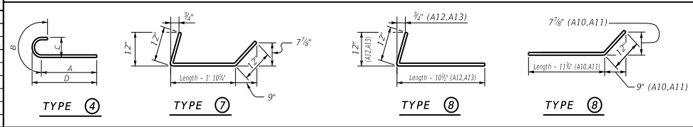
Reinforcement Details
